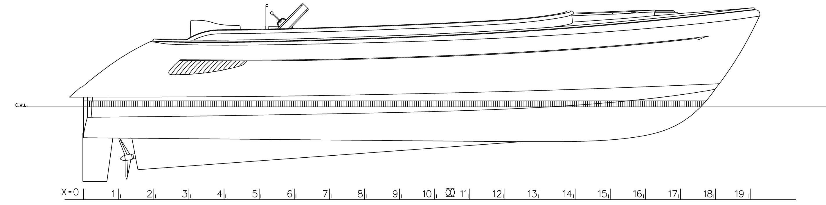
PROFILE VIEW
