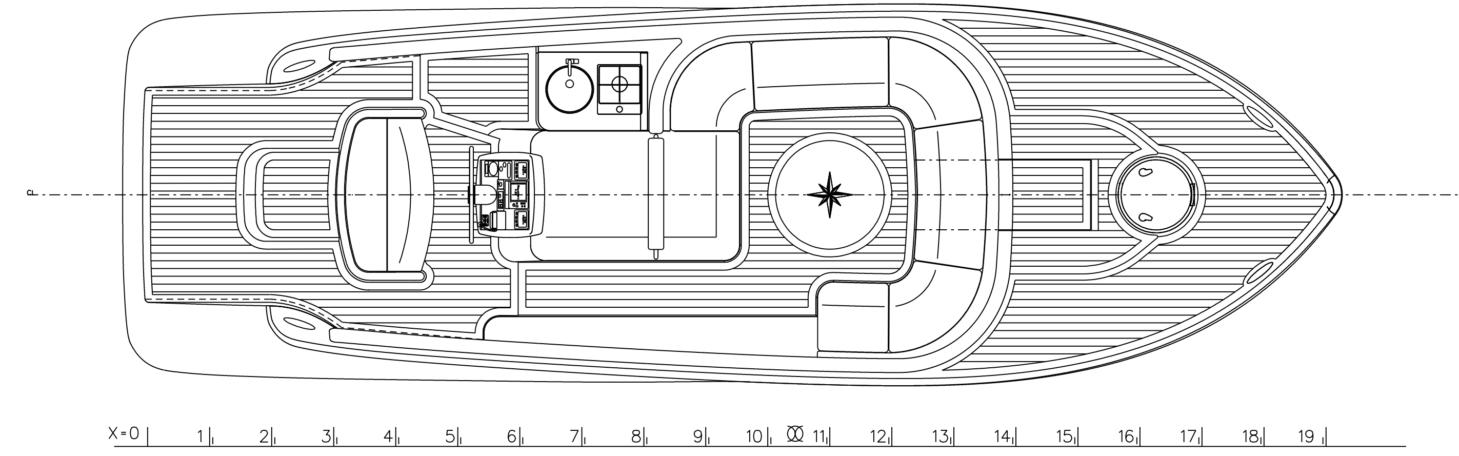
PLAN VIEW
