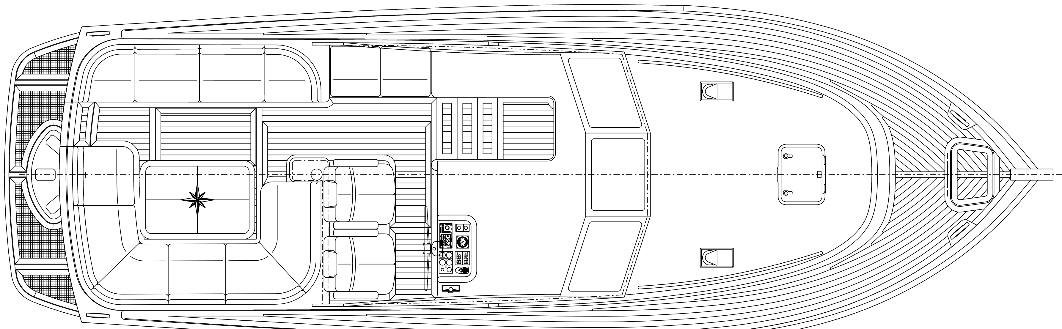
DEK PLAN
