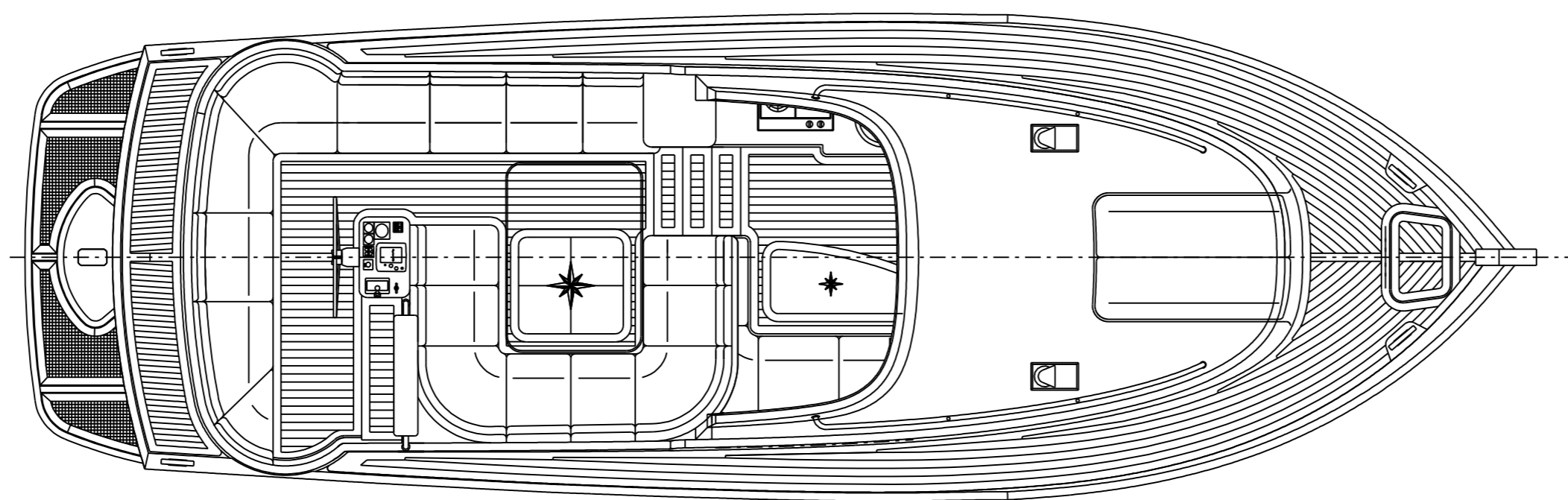
DEK PLAN
